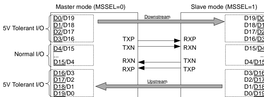
Figure 12 5V tolerant I/O
