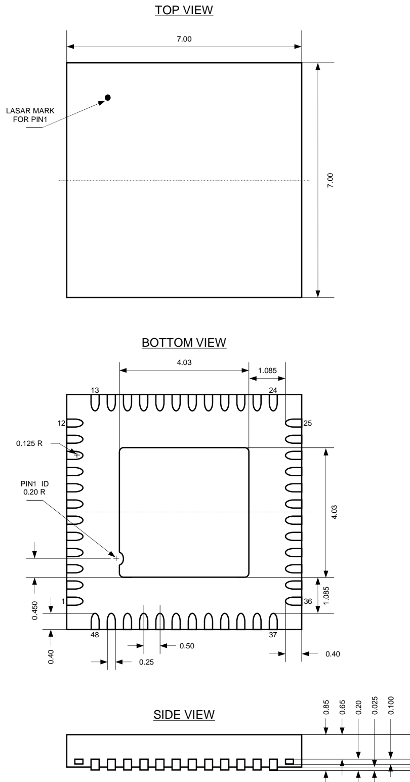
Figure 15 48-pin QFN package physical dimension
