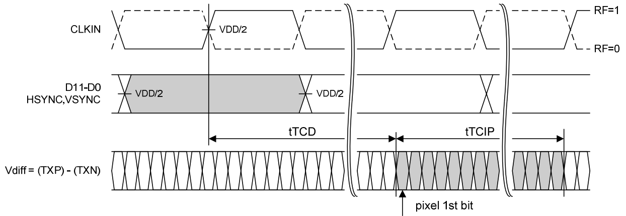
Figure 23. THCV231 Latency
