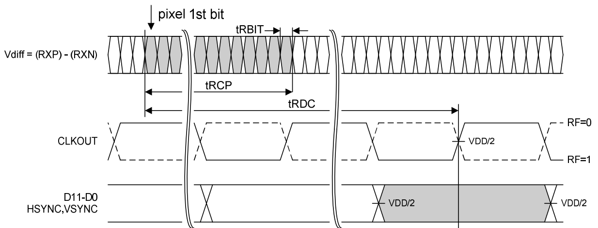
Figure 24. THCV236 Latency
